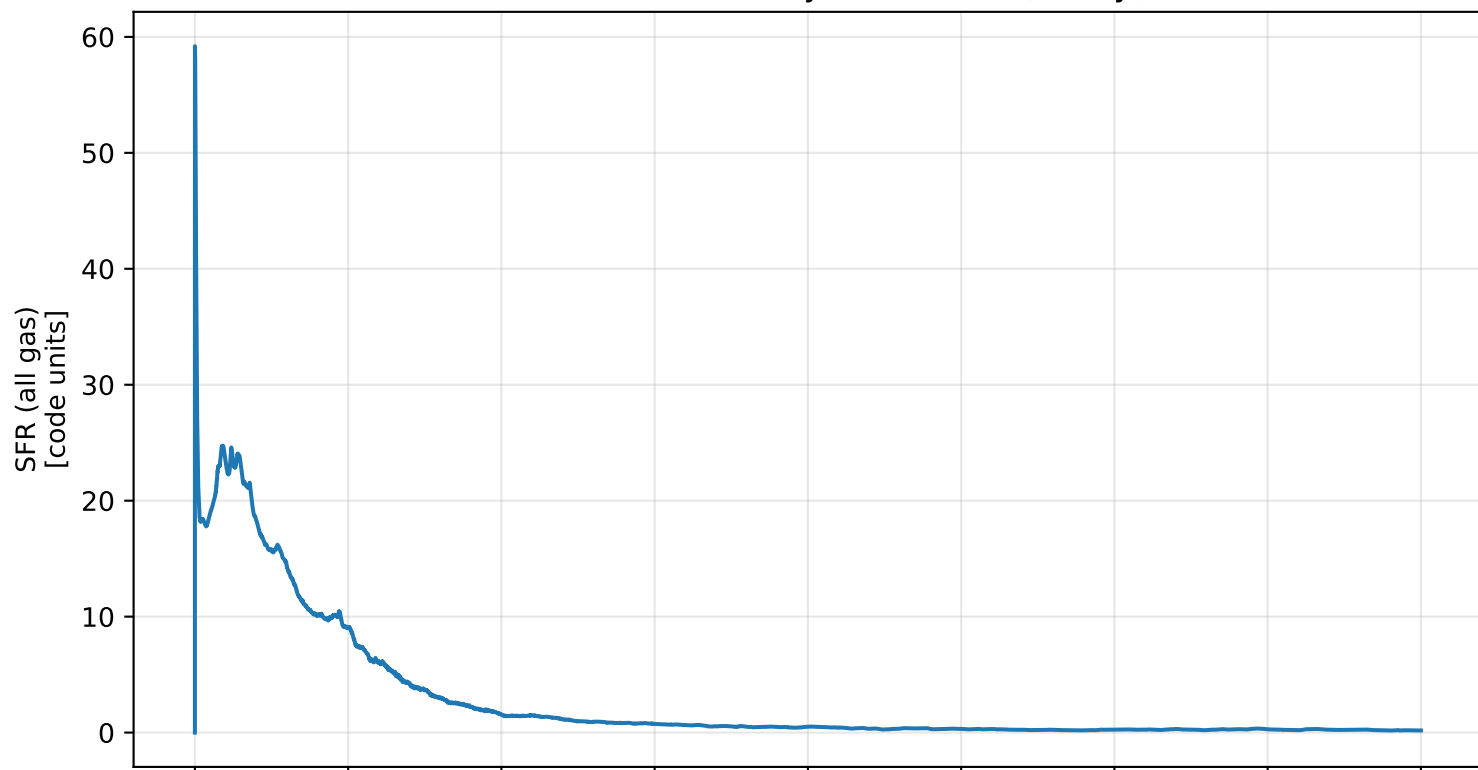
Star formation history - MW + GC (heavy)
