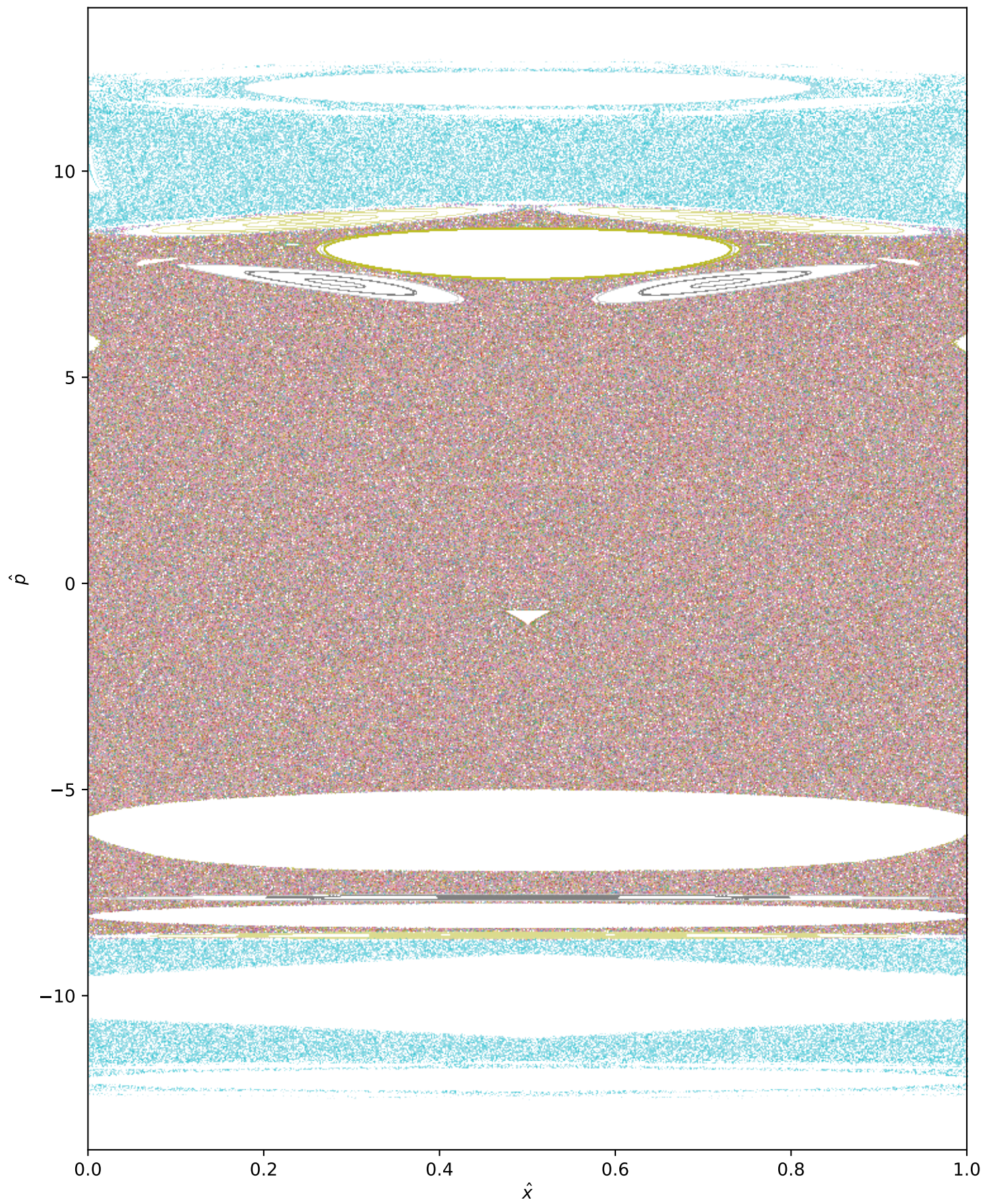
Phase portrait, k = 10 ( x_0 = 0.7300 )
