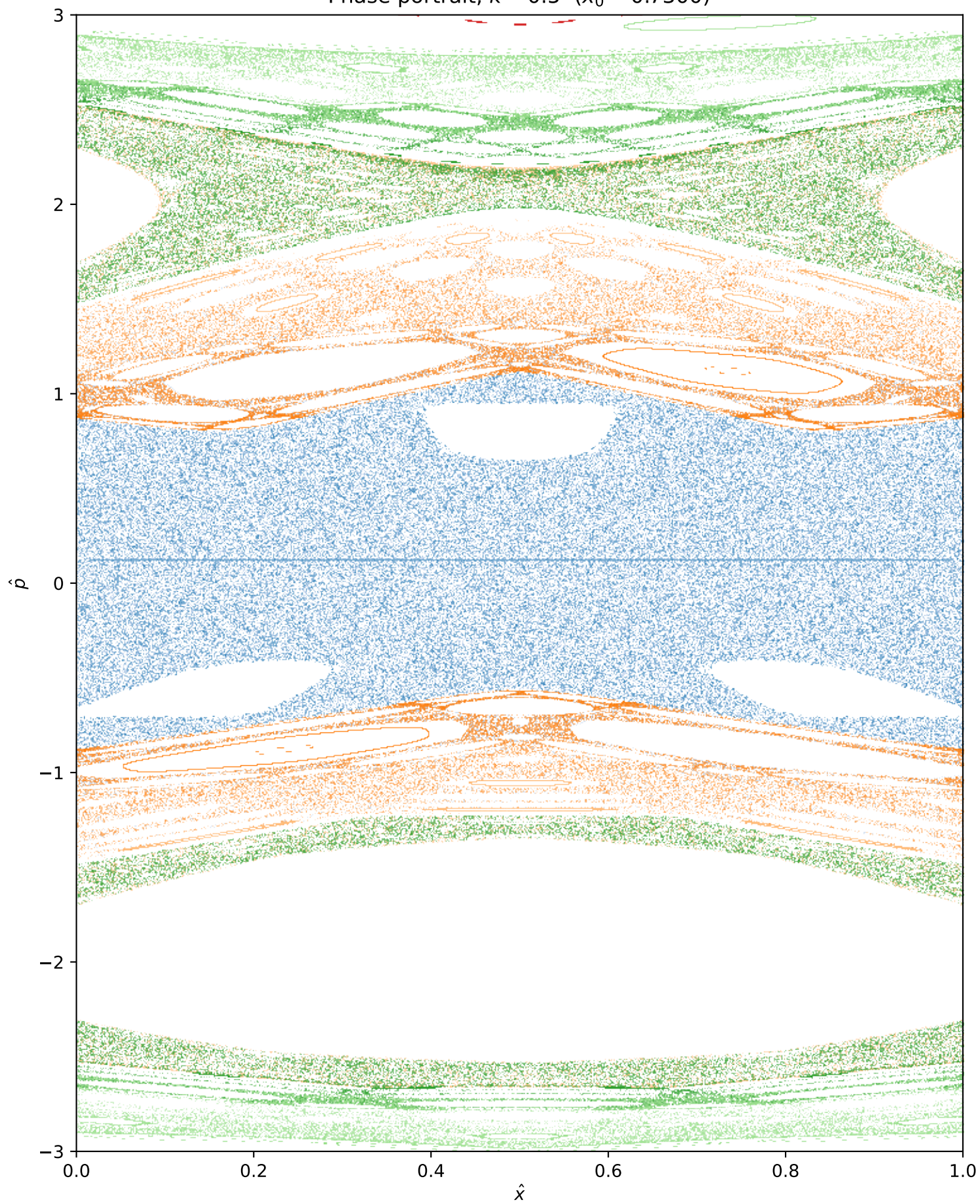
Phase portrait, k = 0.5 ( x_0 = 0.7300 )
