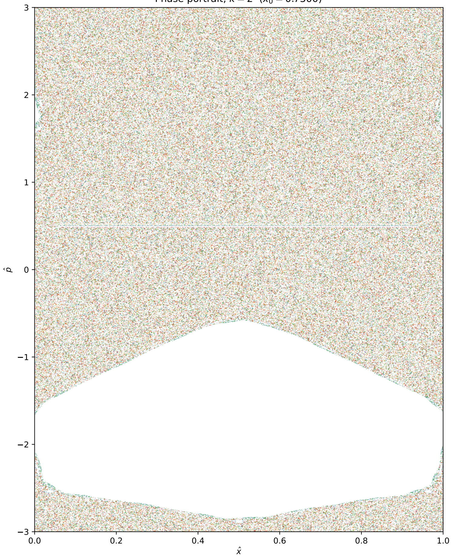
Phase portrait, k = 2 ( x_0 = 0.7300 )
