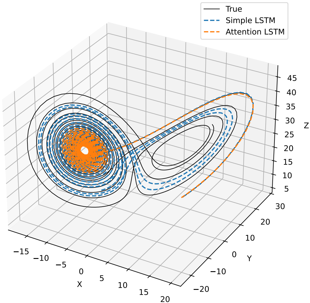
3D Lorenz - True vs Predictions
