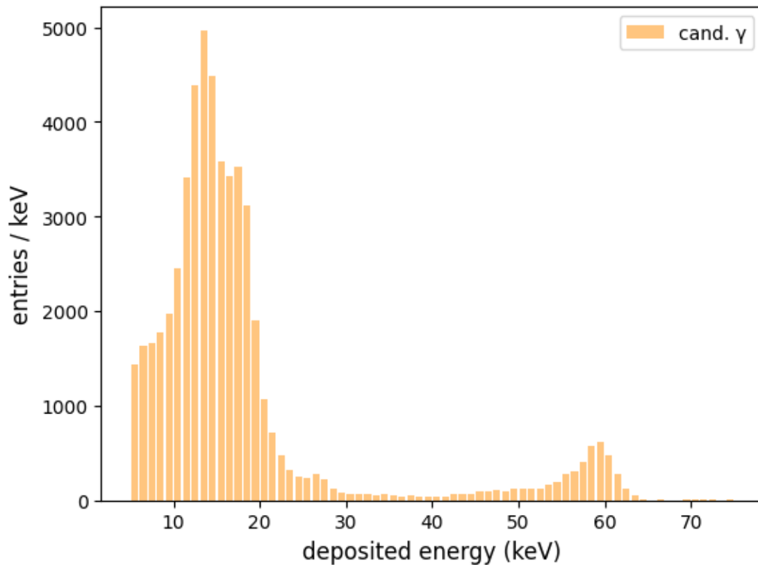
Abbildung 16: from shielded Americium
