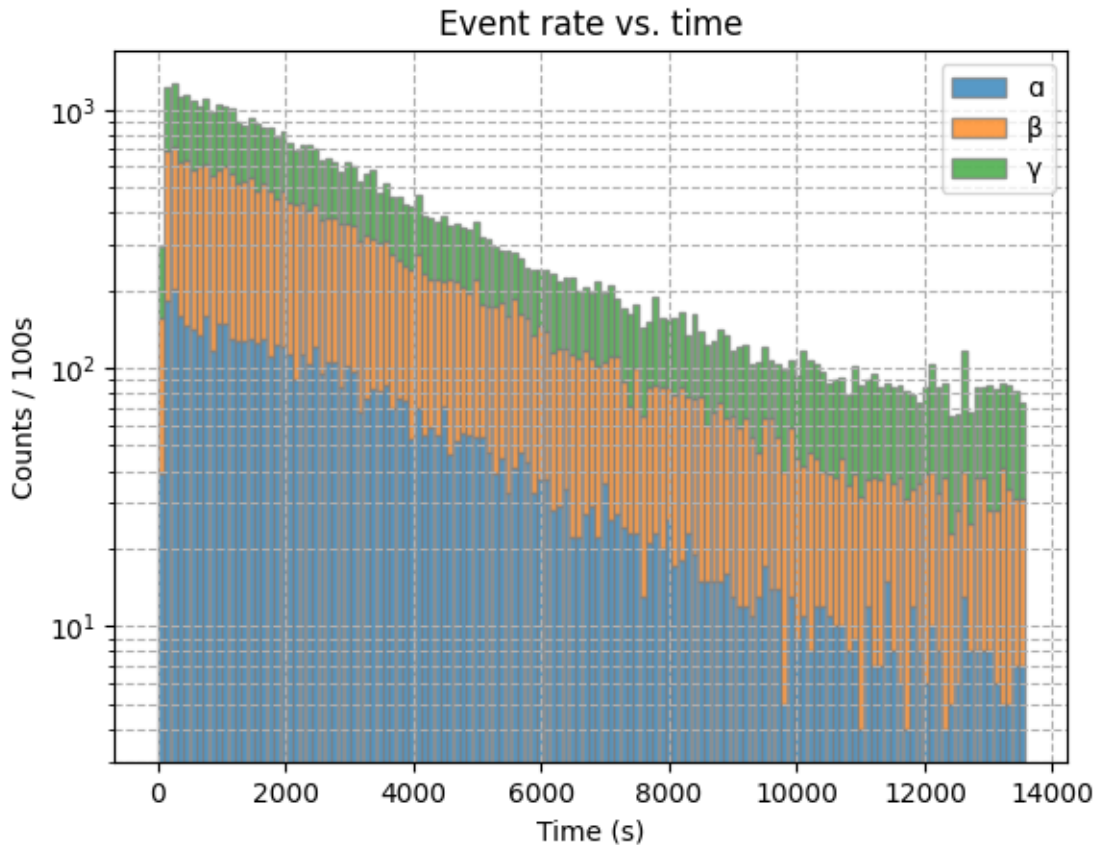
Abbildung 19: Rate of Radon decay products. vs. Time
