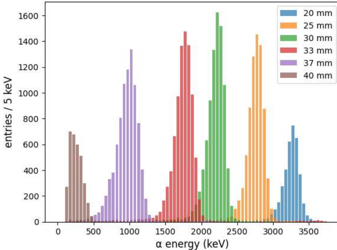
\alpha spectra of a thin Am-241 source for different detector distances
