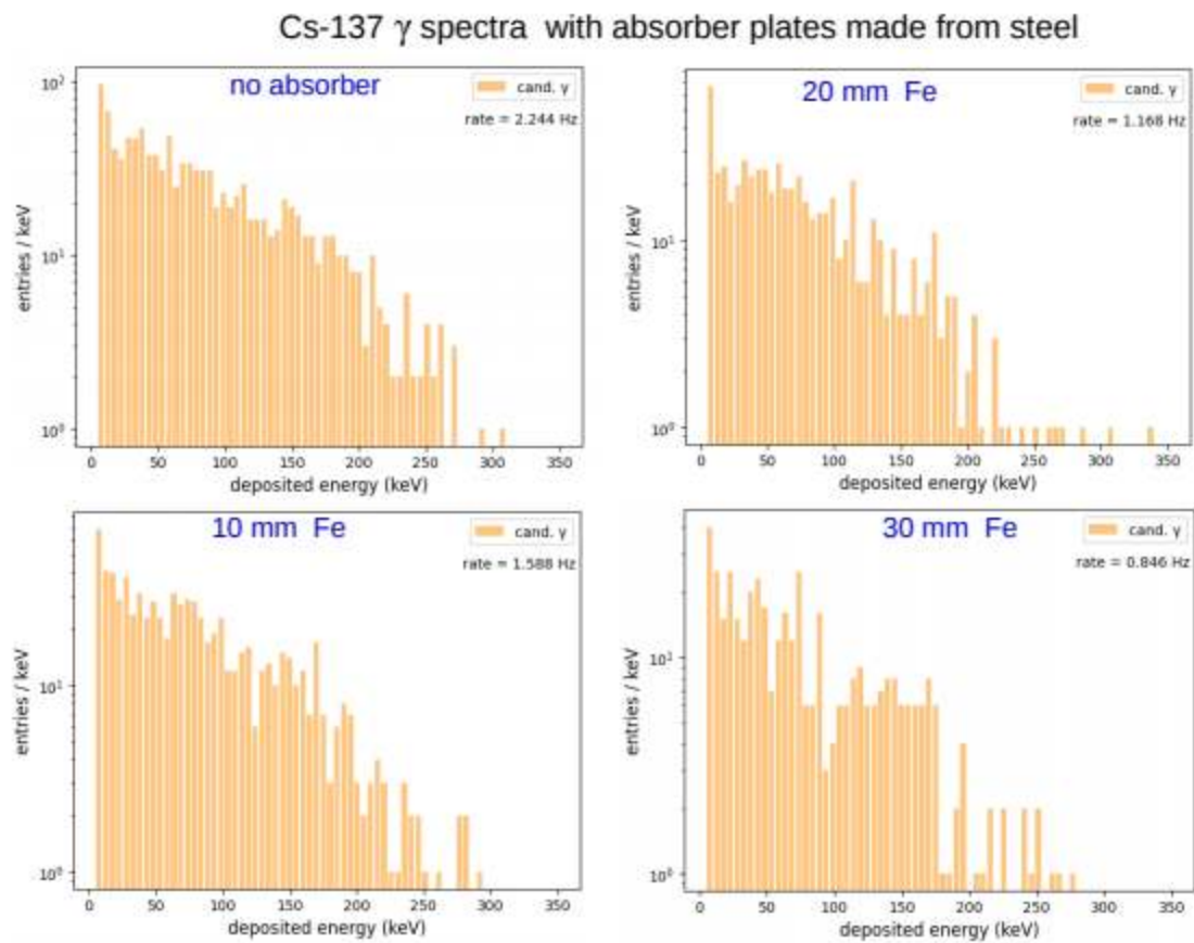
Abbildung 20: Cs-137 \gamma spectra for different thickness of Fe absorber plates
