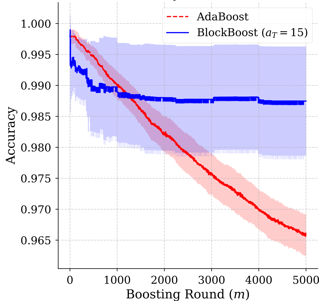
Test Accuracy (Clean Holdout)
