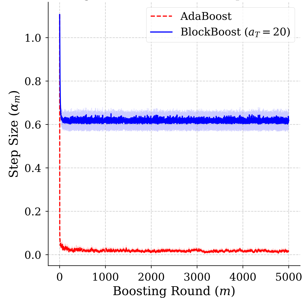
Algorithm Momentum (Step Size)
