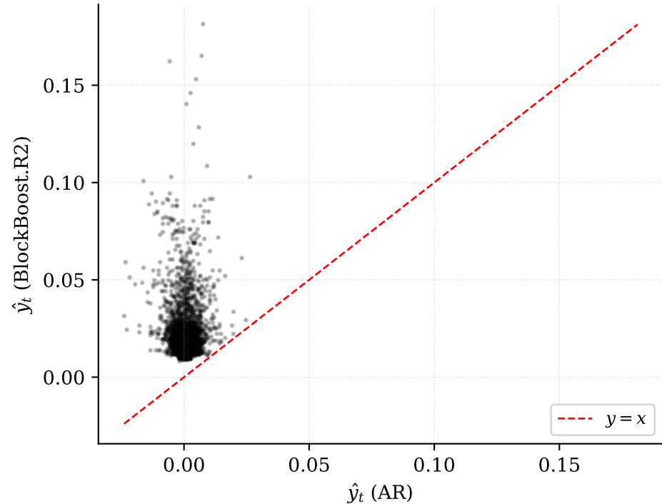
AR vs. \ BlockBoost.R2 Predictions
