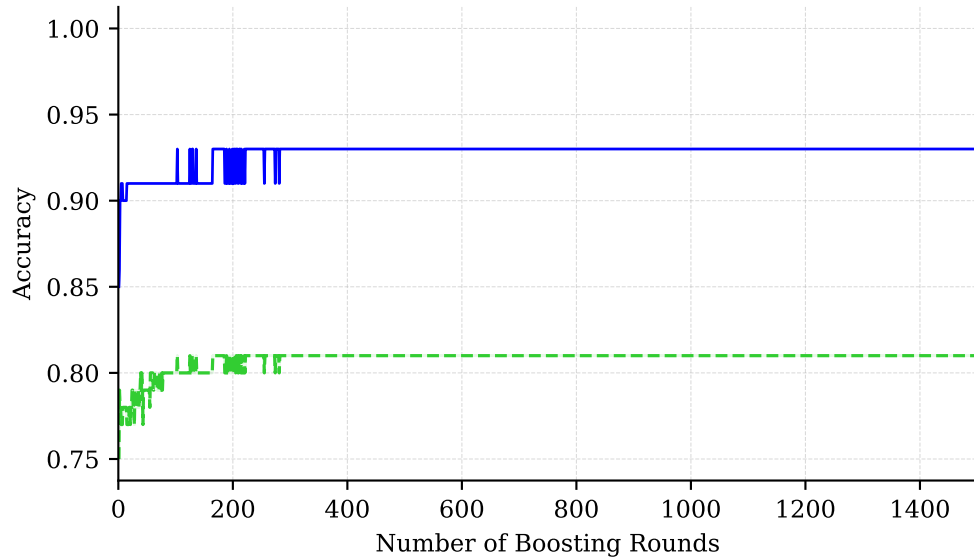
BlockBoost ( a_T = 10 ) — ECG200
