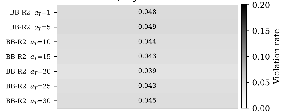
Violation Rate \alpha = 0.05 (target = 0.05)
