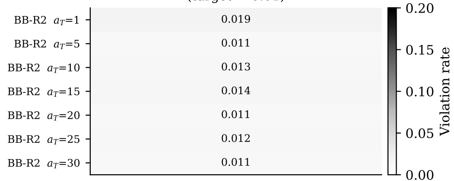
Violation Rate \alpha = 0.01 (target = 0.01)
