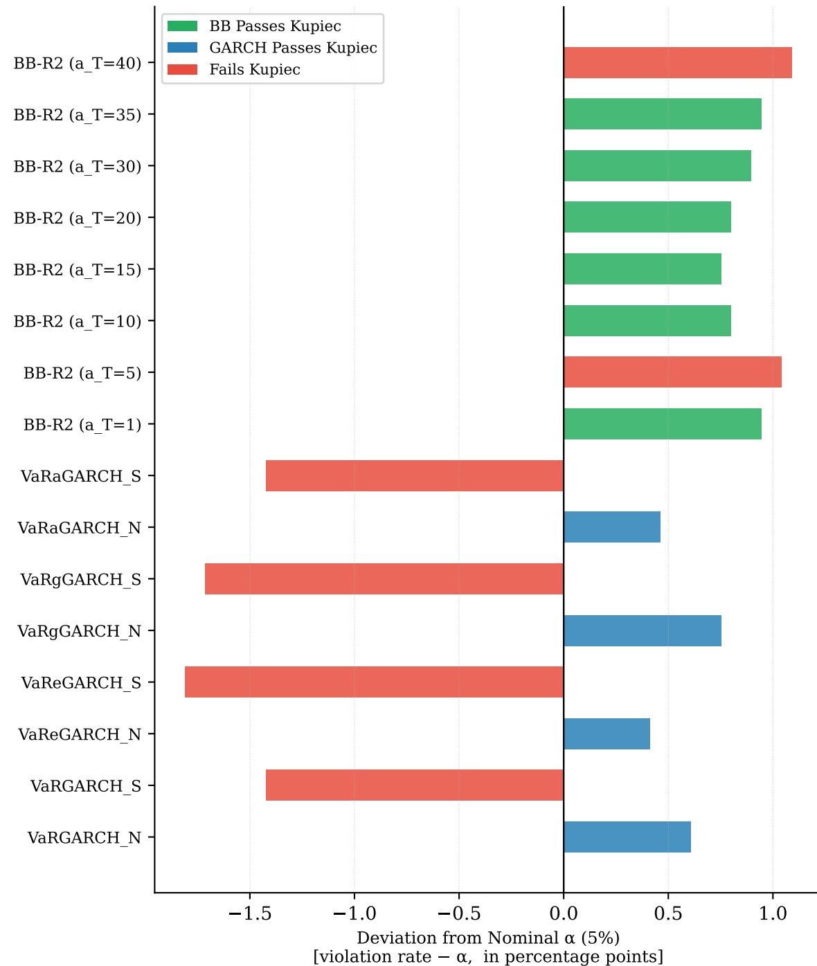
\alpha = 5\% Violation Rate Distance
