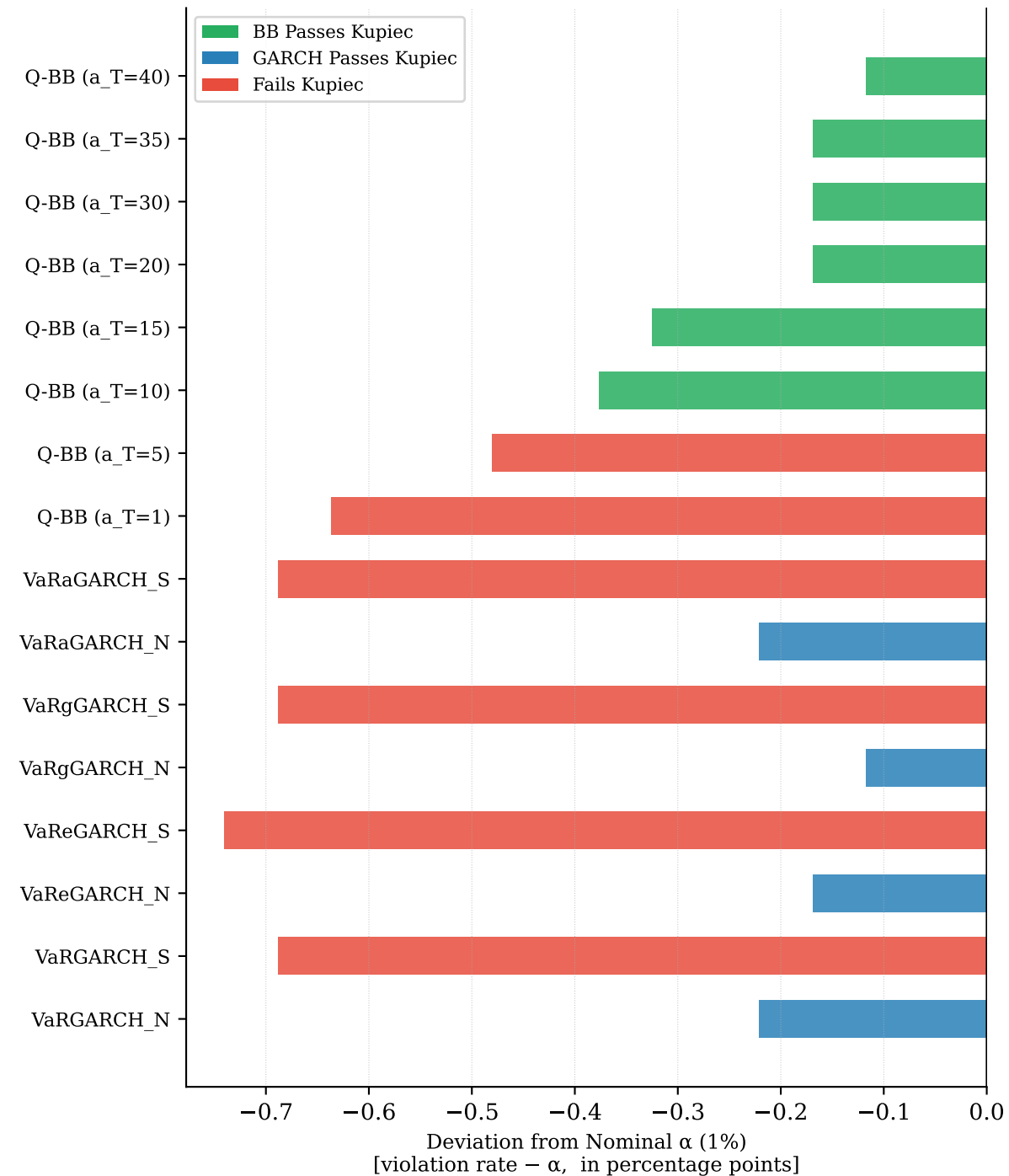
\alpha = 1\% Violation Rate Distance
