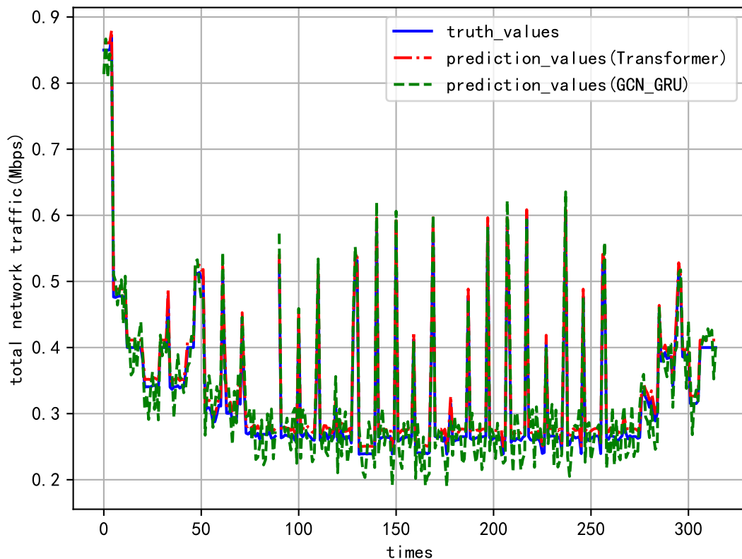
Network Total Traffic Prediction Curve
