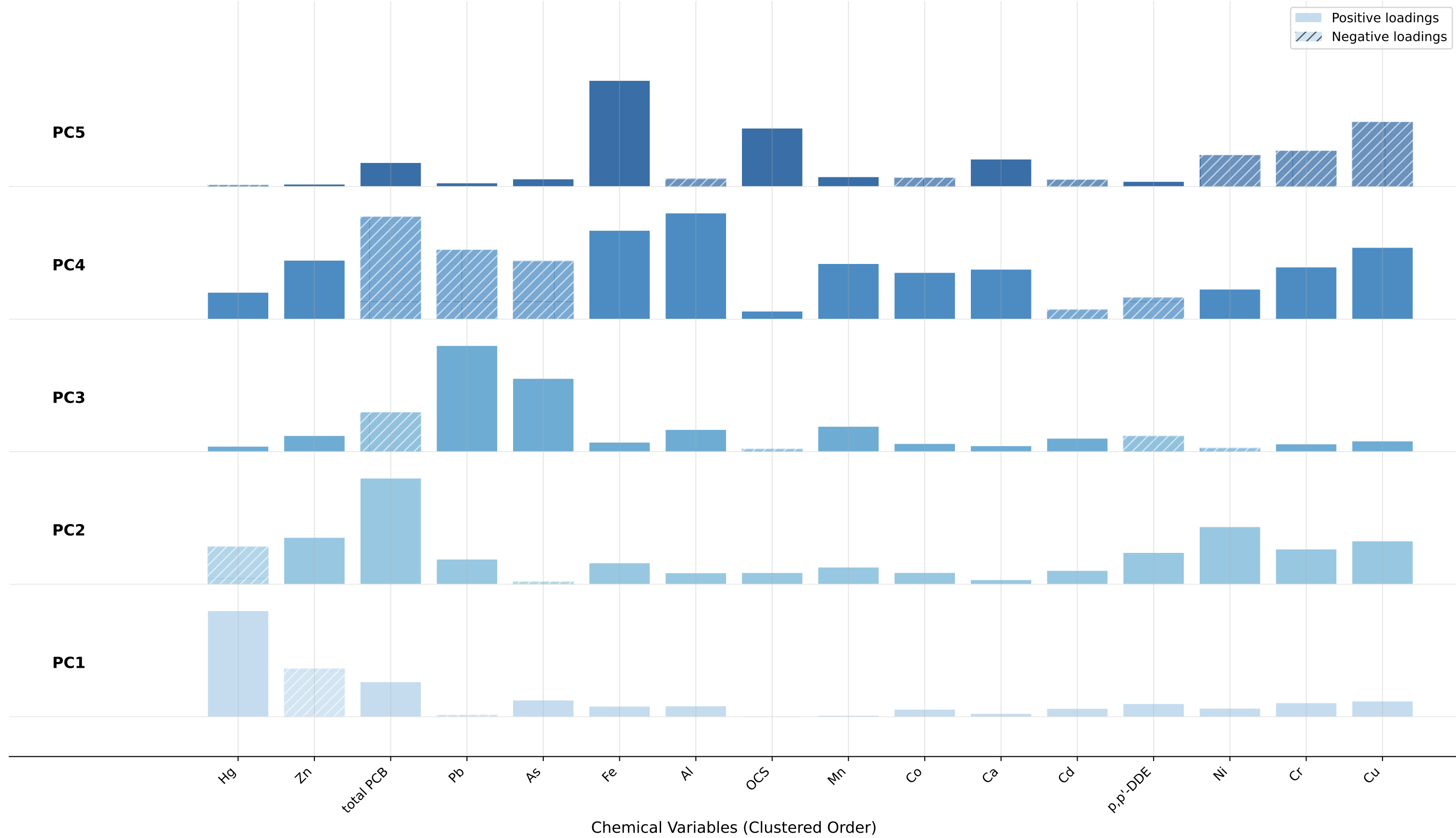
PC Loadings Ridge Plot (Variables Ordered by Hierarchical Clustering)
