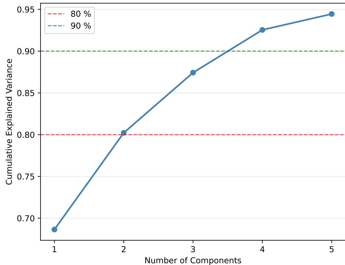
Cumulative Variance
