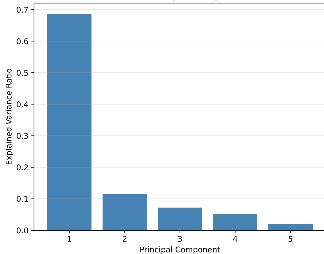
Variance Explained per PC
