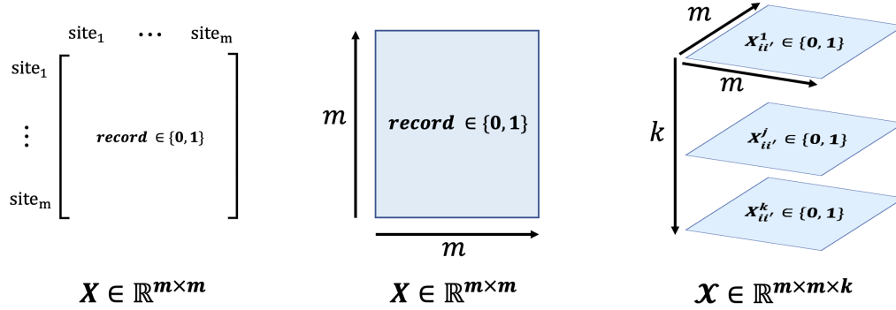
Figure 2.8: Co-assignment matrix \mathbf{X}_{m \times m} (left and middle) does not show which cluster a record refers to. Redistribute its records into a tensor \mathcal{X}_{m \times m \times k} (right), the third dimension ticked by cluster labels. \mathcal{X}_{ii'j} indicates whether objects i and i' are co-assigned into the j -th cluster.
