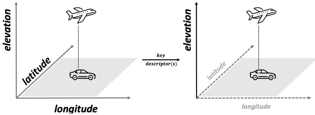
Figure 2.4: Not all descriptors help separate a small number of classes. An aircraft and a car are barely distinguishable on the horizontal descriptors (longitude, latitude), yet a single key descriptor—elevation—separates them cleanly. When only a few classes must be told apart, the right descriptor subset matters more than the number of descriptors, and retaining irrelevant ones only adds noise.
