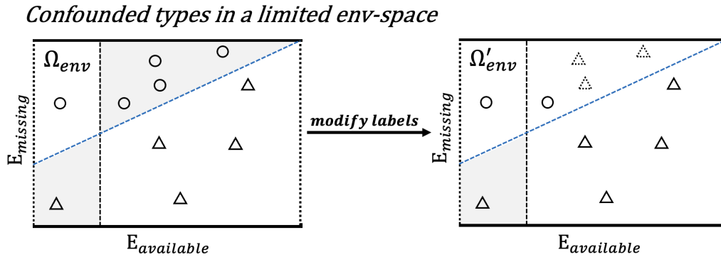
Figure 2.3: Confounded community types in a limited environmental space. The true boundary (blue dashed) depends on an unobserved feature E_{missing} , leaving the types overlapping (shaded) on the available features E_{available} . The original approach relabels part of C_1 as C_2 in one direction only ( \Omega_{env} \rightarrow \Omega'_{env} , dotted triangles), reducing but not removing the overlap—separability bought by altering true labels.
