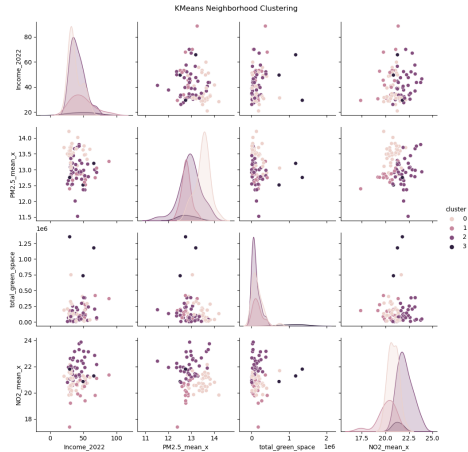
Figure 2: KMeans Clusters
