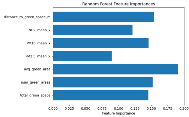
Figure 7: Feature importance by Random Forest Regressor (duplicate of Figure 1)
