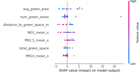
Figure 4: SHAP Values by Gradient Boosting Regressor
