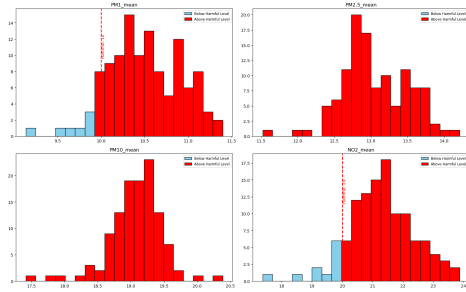
Figure 6: Average \text{PM}_{2.5} per Neighborhood
