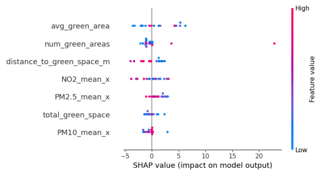
Figure 10: SHAP Values by Gradient Boosting Regressor (duplicate of Figure 4)
