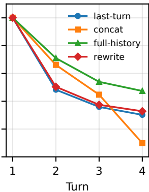
BM25 (lexical)
