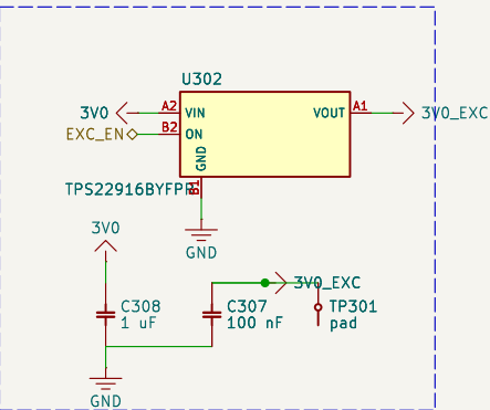
Excitacao chaveada TPS22916
