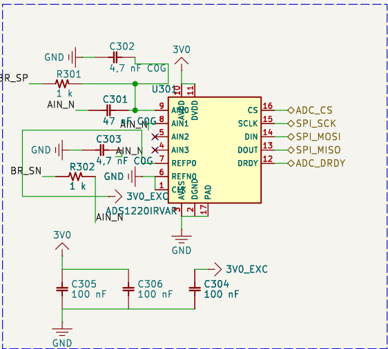
Conversor ADS1220
