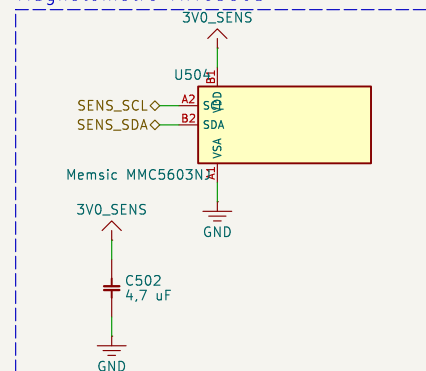
Magnetometro MMC5603
