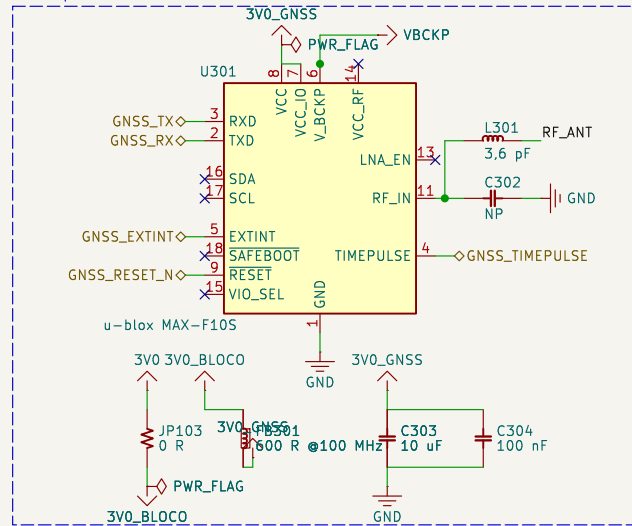
Receptor MAX-F10S
