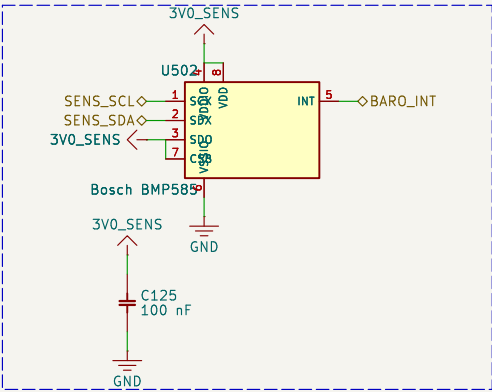
Barometro BMP585
