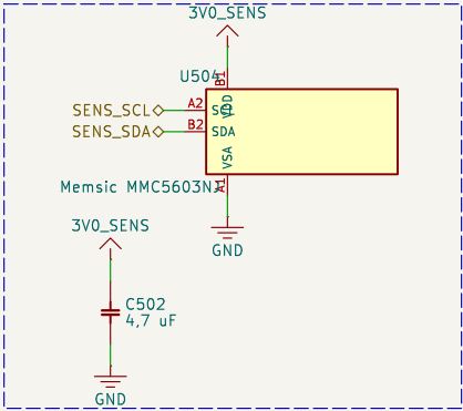
Magnetometro MMC5603
