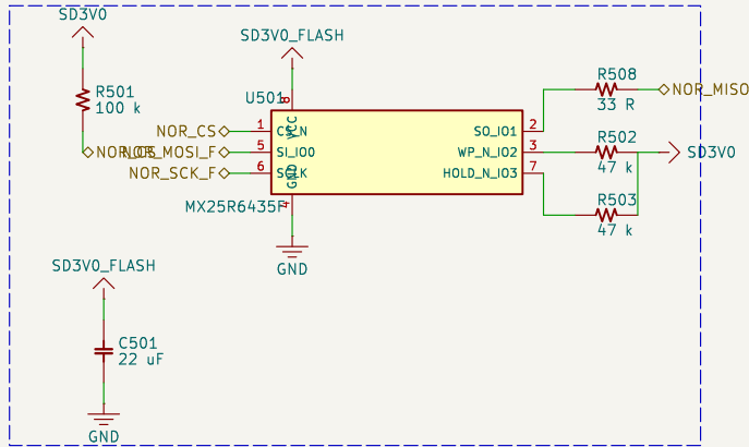
Flash NOR MX25R6435F
