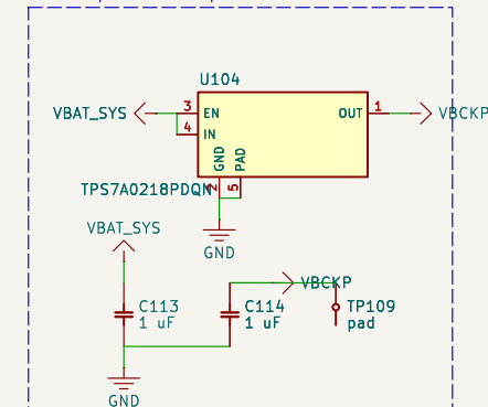
Backup do receptor GNSS
