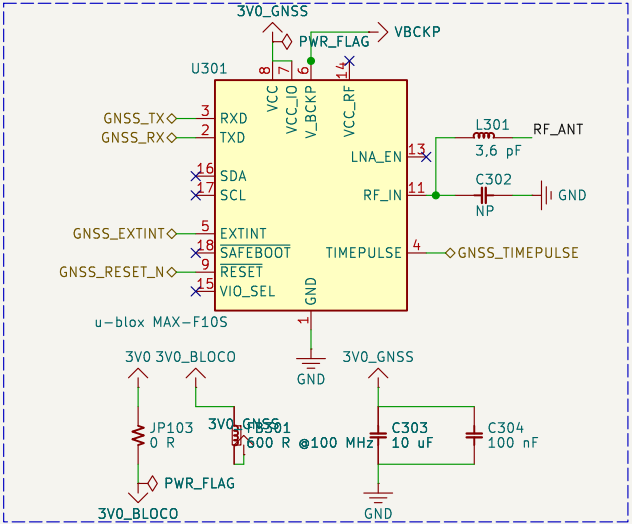
Receptor MAX-F10S
