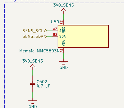
Magnetometro MMC5603
