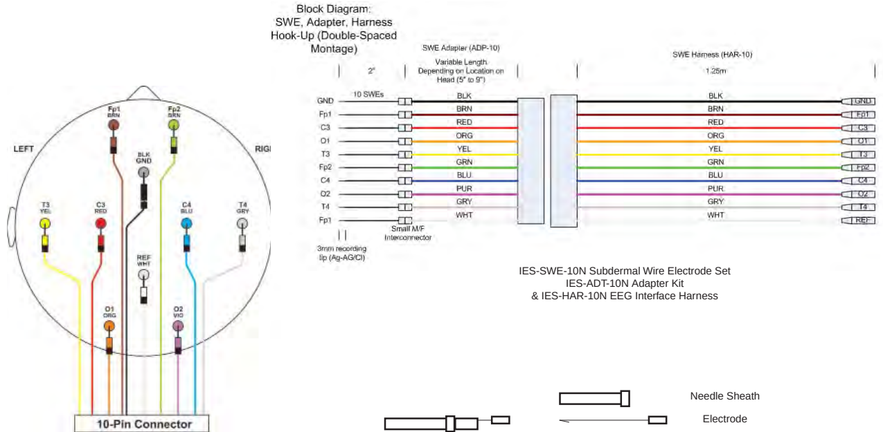
IES-SWE-10N Subdermal Wire Electrode Set & IES-ADT-10N Adapter Kit
