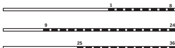
QG36B-SP10X-000 36-contact, macro-micro strip
