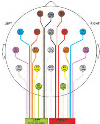
IES-CPE-20N Conductive Plastic Electrode Set Electrode Placement - 10:20 System
