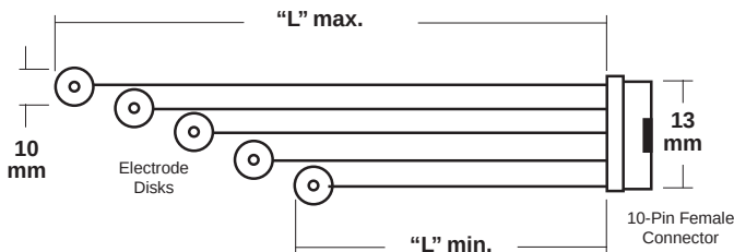
IES-CPE-20N Conductive Plastic Electrode Set
