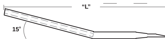
Bent single-tail passing needle Catalog No. BPNK1-10X or BPN2K1-10X
