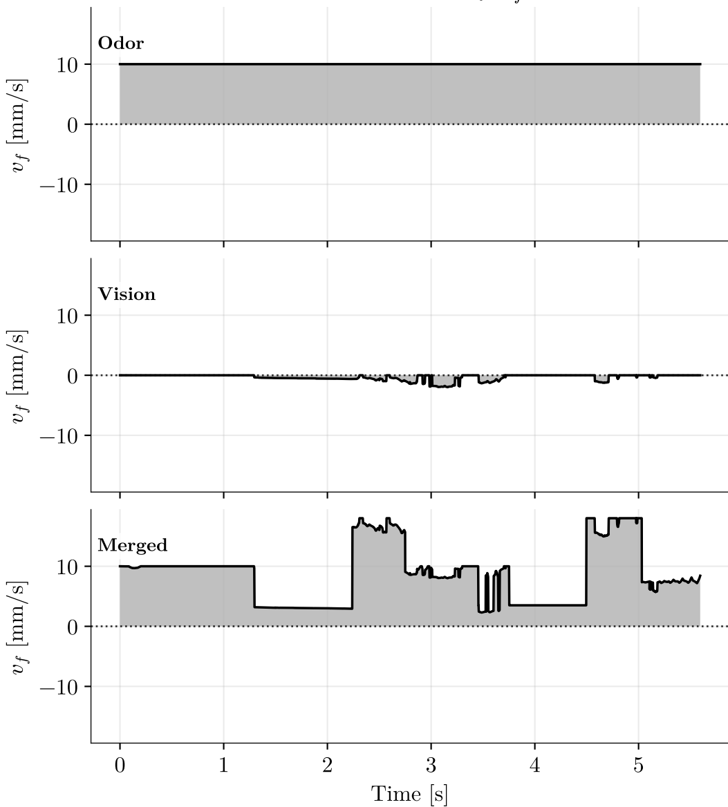
Forward velocity v_f
