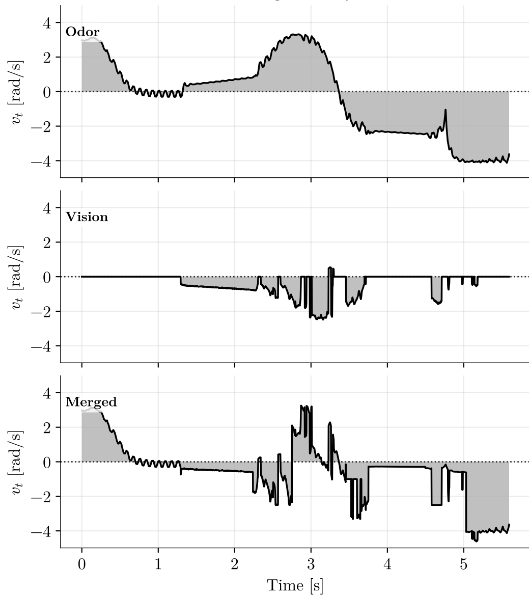
Turning velocity v_t
