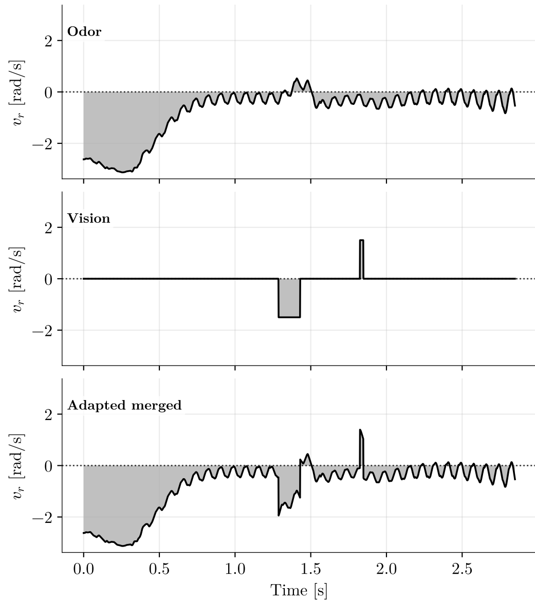
Yaw velocity v_r
