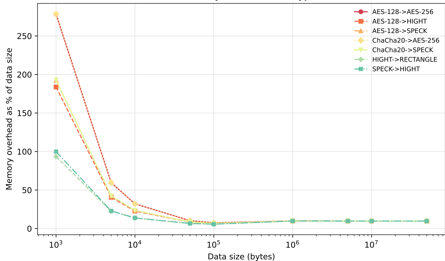
Phase 3+4 combined — Memory overhead (encryption) as % of data size
