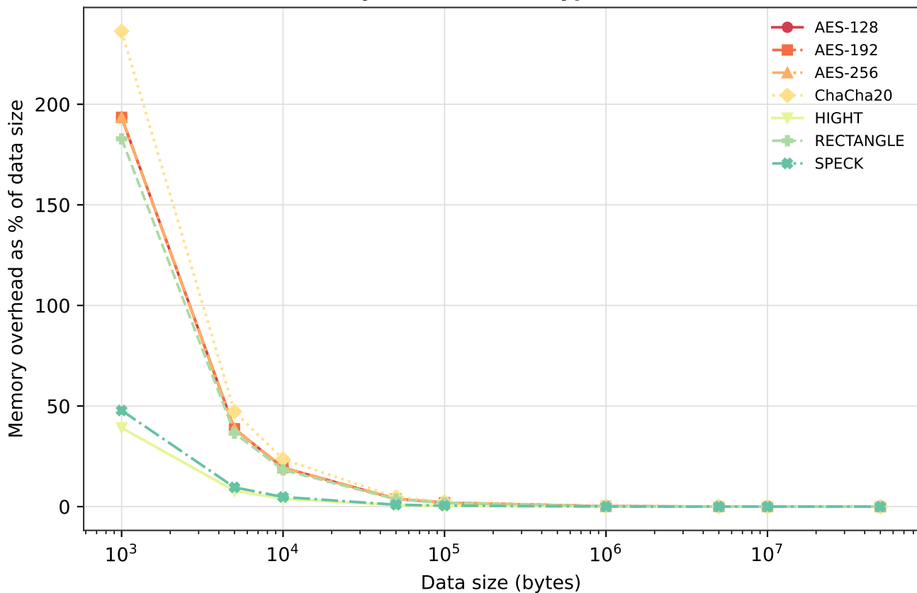
Phase 1 — Memory overhead (encryption) as % of data size
