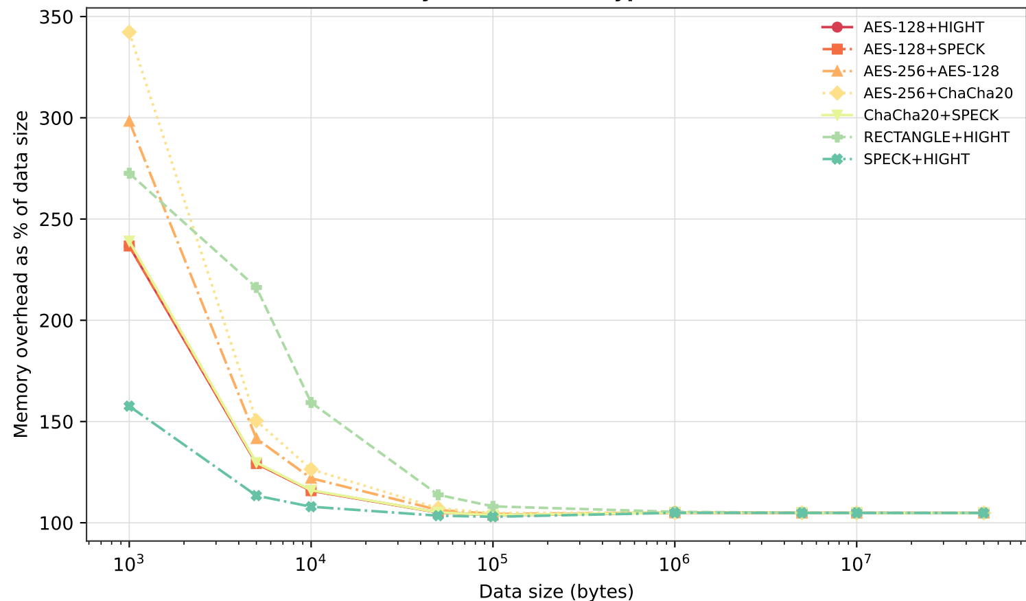
Phase 2 — Memory overhead (encryption) as % of data size
