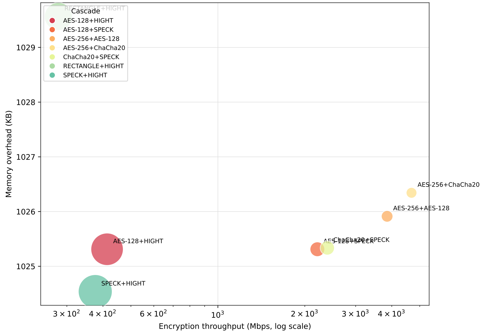
Phase 2 — Throughput vs. memory overhead at 1MB
