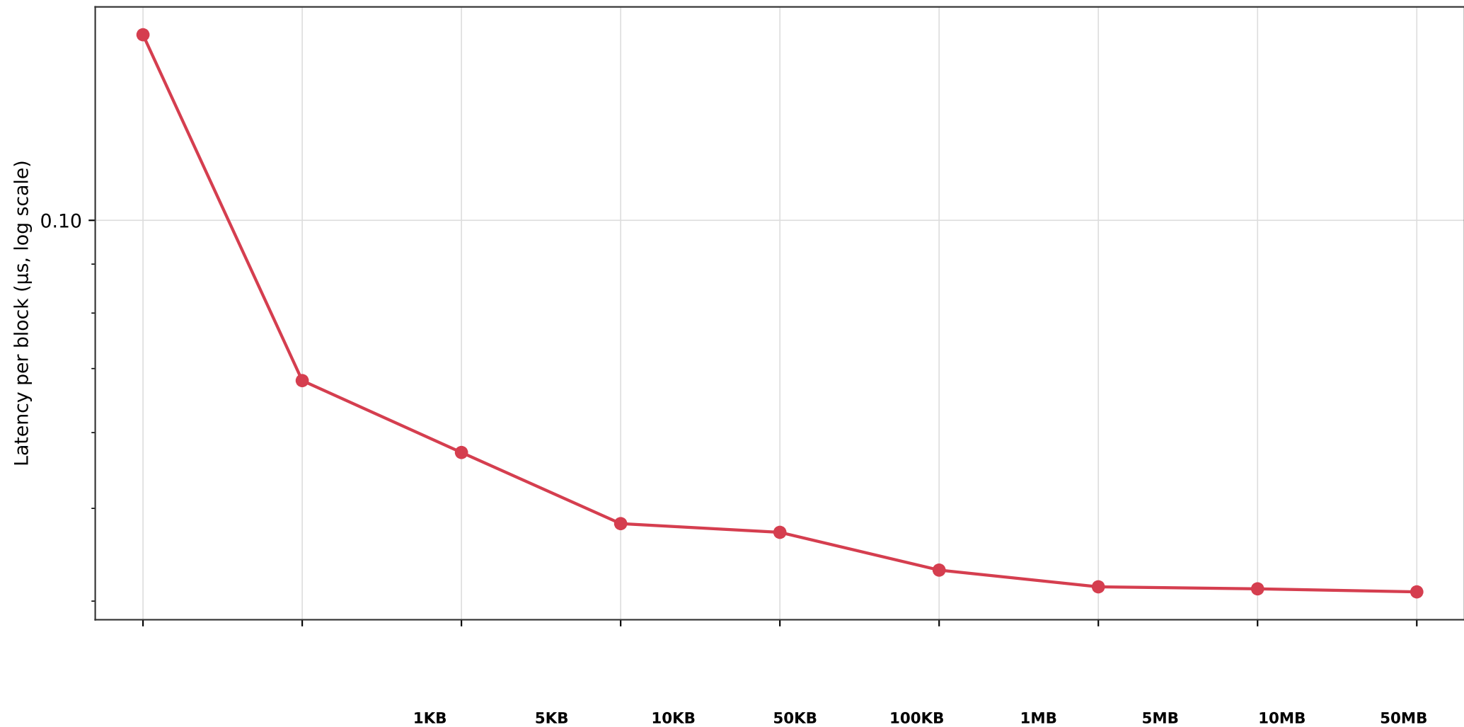
Phase 3 — Per-block latency (AES-256+ChaCha20+AES-128) by packet size
