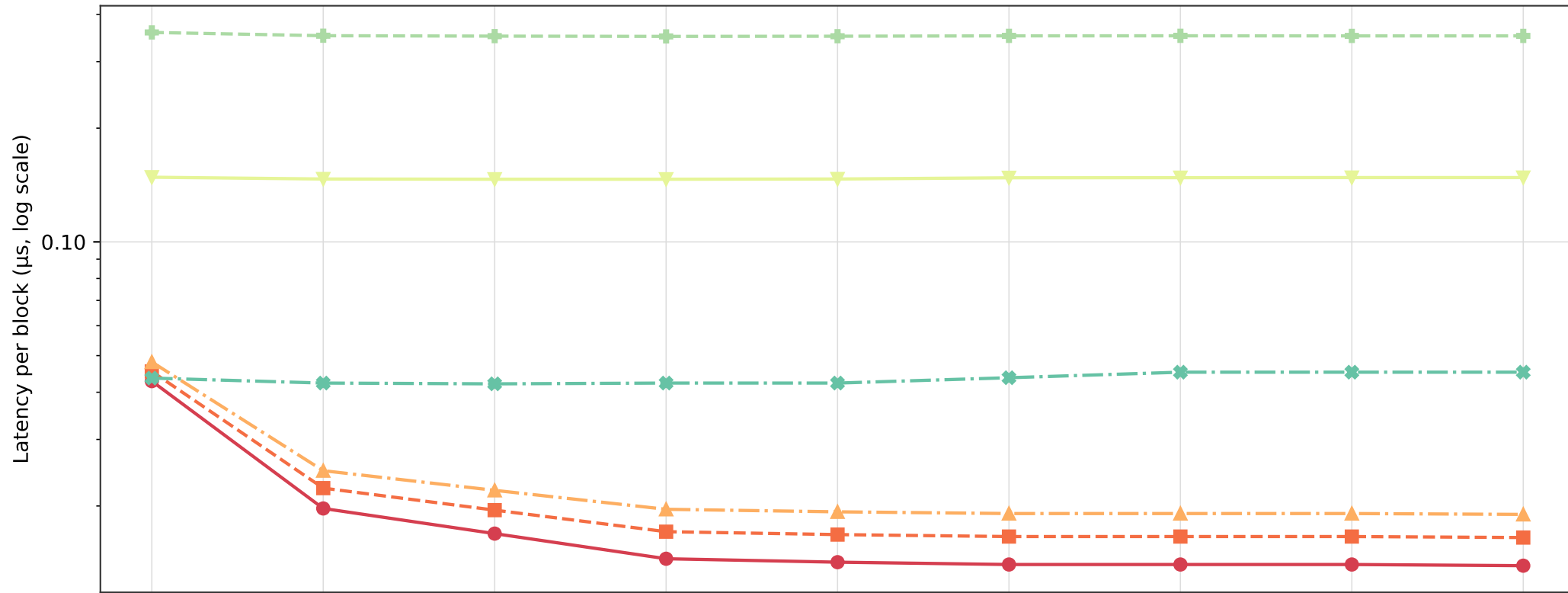
Phase 1 — Per-block latency by cipher and packet size
