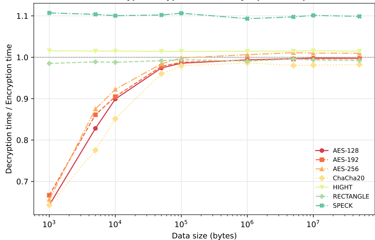
Phase 1 — Decrypt/Encrypt time ratio by cipher and packet size
