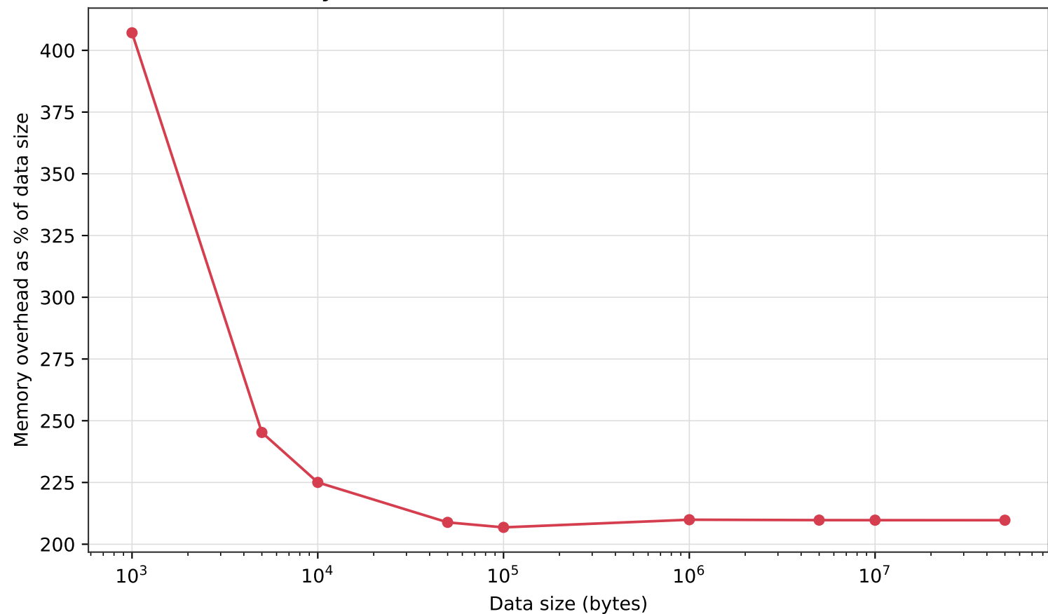
Phase 3 — Memory overhead as % of data size (AES-256+ChaCha20+AES-128)
