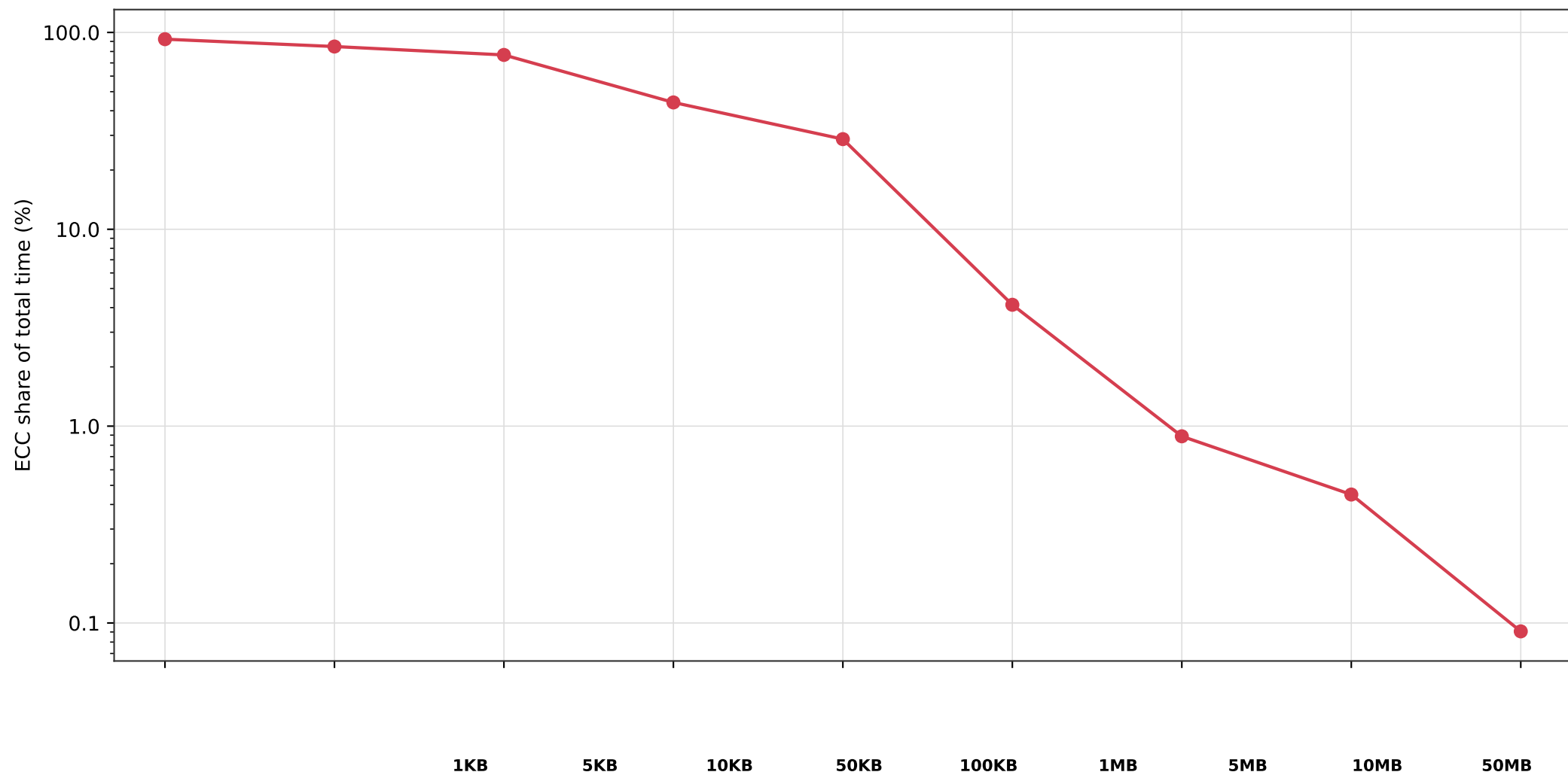
ECC handshake share of total time (triple cascade + ECC) by packet size
