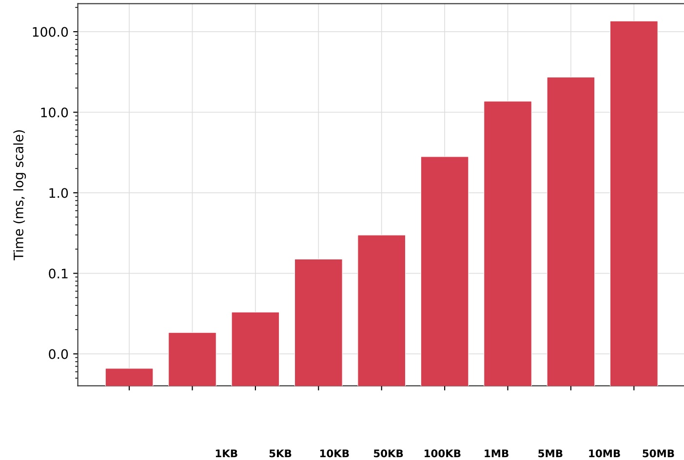
Decryption time
