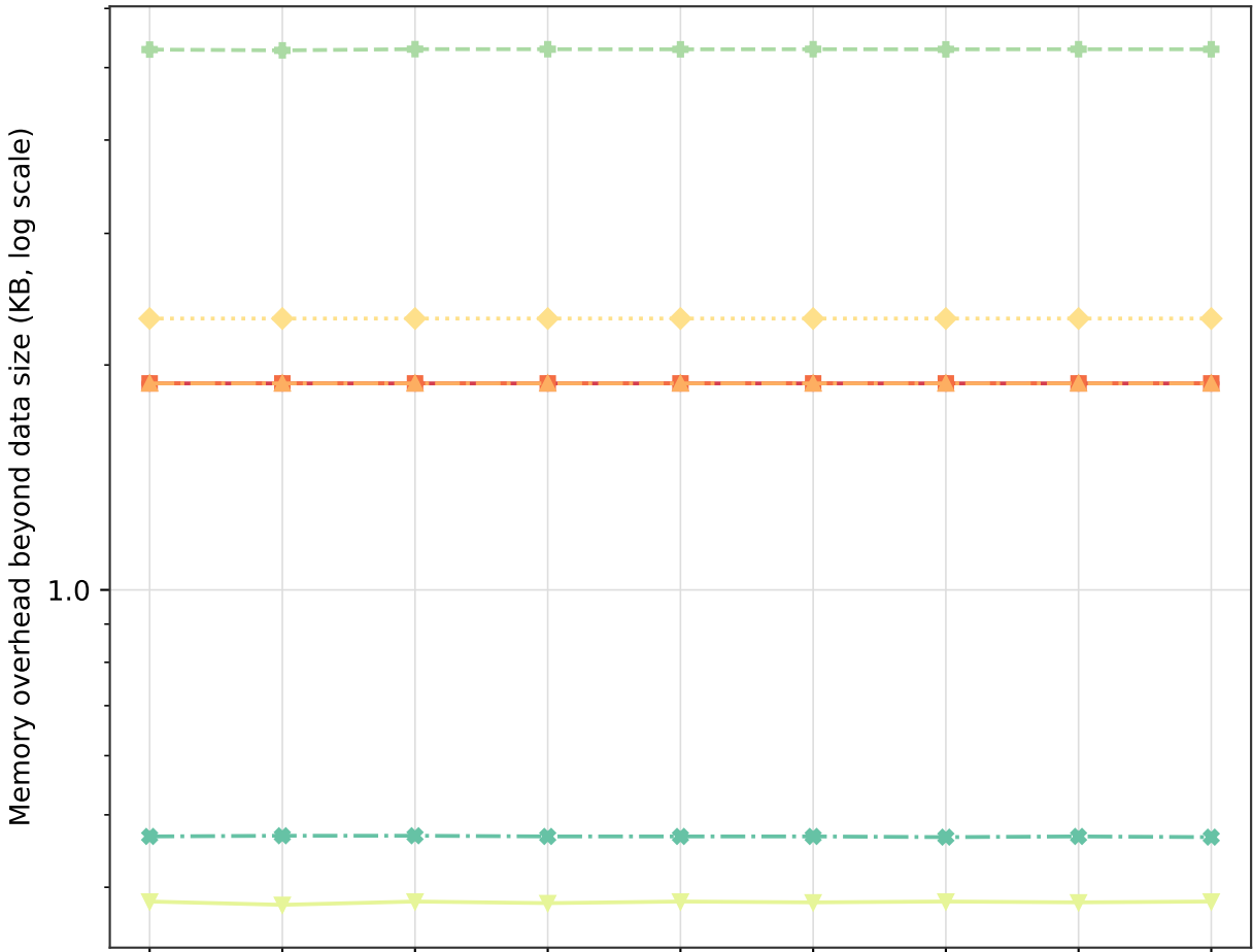
Encryption
