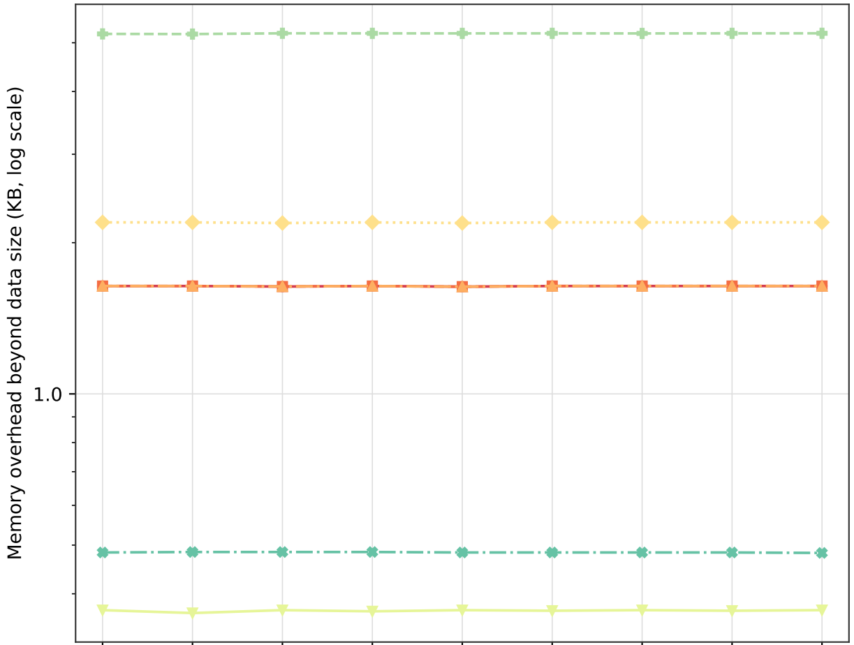
Decryption
