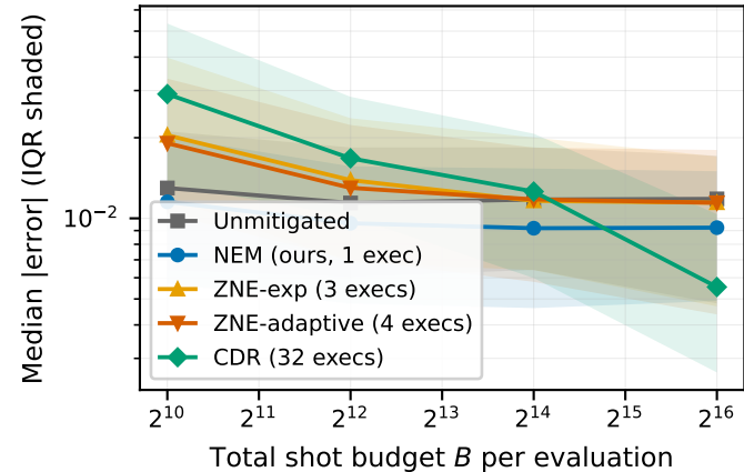
Stochastic device noise
