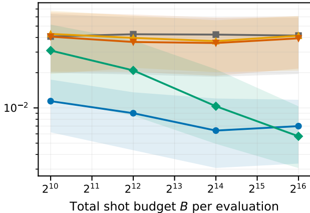
Stochastic + coherent miscalibration
