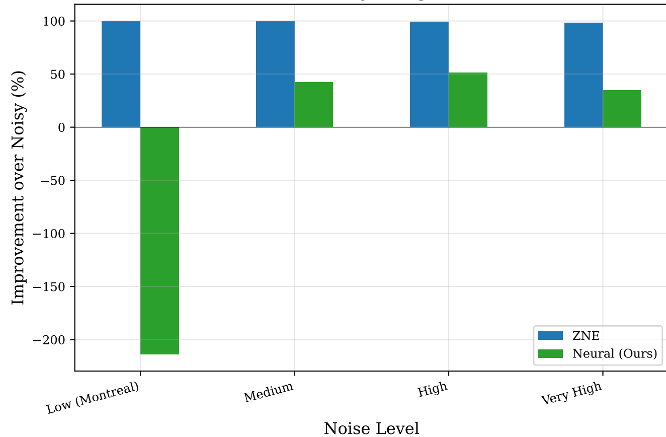
Error Reduction by Mitigation Method
