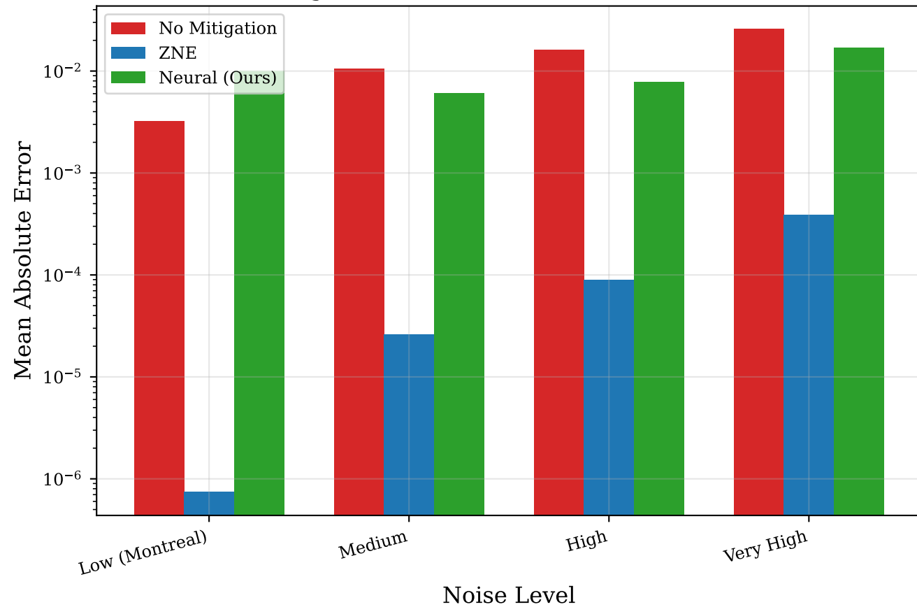
Error Mitigation Performance Across Noise Levels
