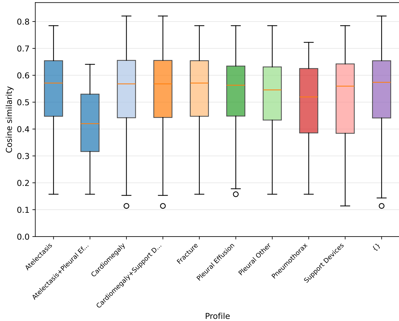
Iteration 100
