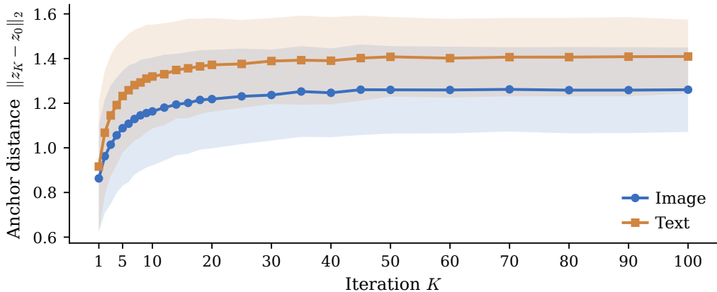
Anchor distance saturates by K \sim 10 , then stays bounded
