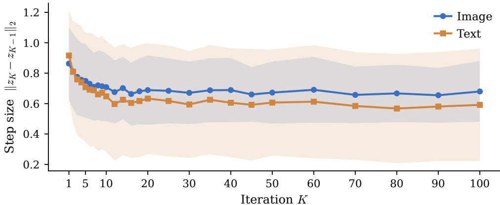
Per-iteration step size: small and bounded across the horizon
