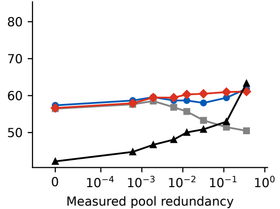
(b) FiQA-2018 (multi-evidence)
