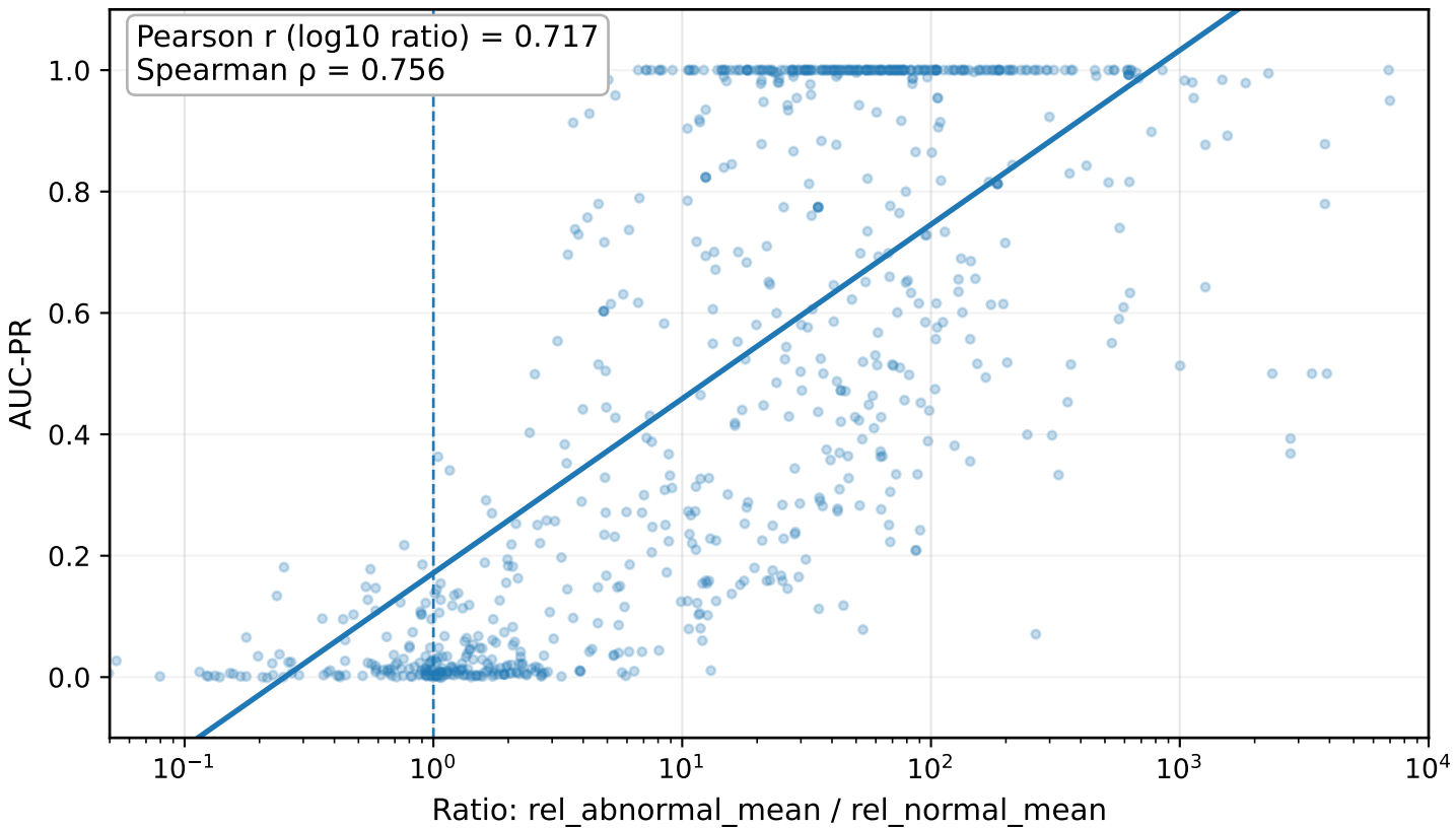
AUC-PR vs relative-error ratio
