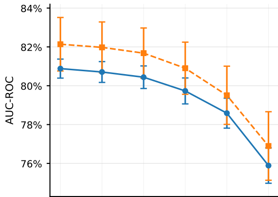
DLiner TimesNet
