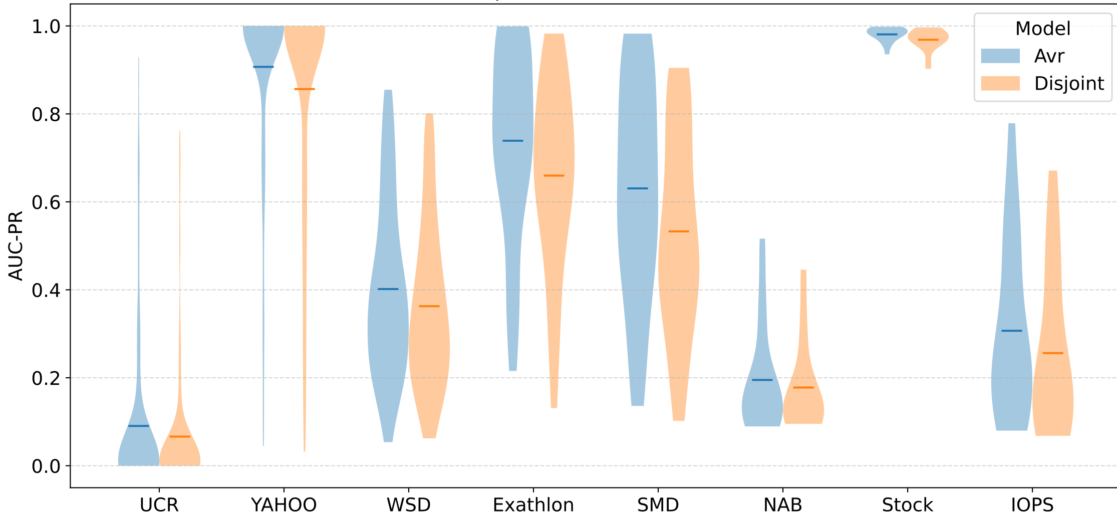
Performance Comparison Across Models and Datasets
