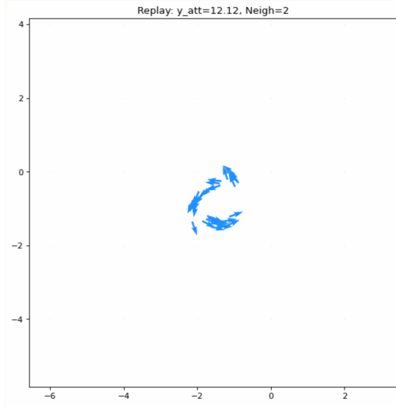
Fig. 2. Visual representation of a successful milling phase emerged from the GA optimization. The drones (blue vectors) exhibit stable circular motion around the swarm’s barycenter while maintaining strict collision avoidance constraints.
