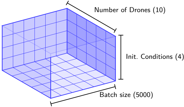
Fig. 1. 3D Tensor structure used for parallel swarm evaluation in PyTorch.
