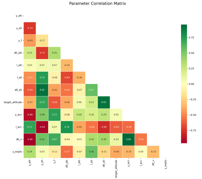
Fig. 3. Parameter correlation matrix generated from the unique global optimums across all tested swarm sizes ( N = 10 to 30 ). The diverging color scale highlights the true macroscopic scaling laws and physical trade-offs required to sustain the milling phase at any scale.
