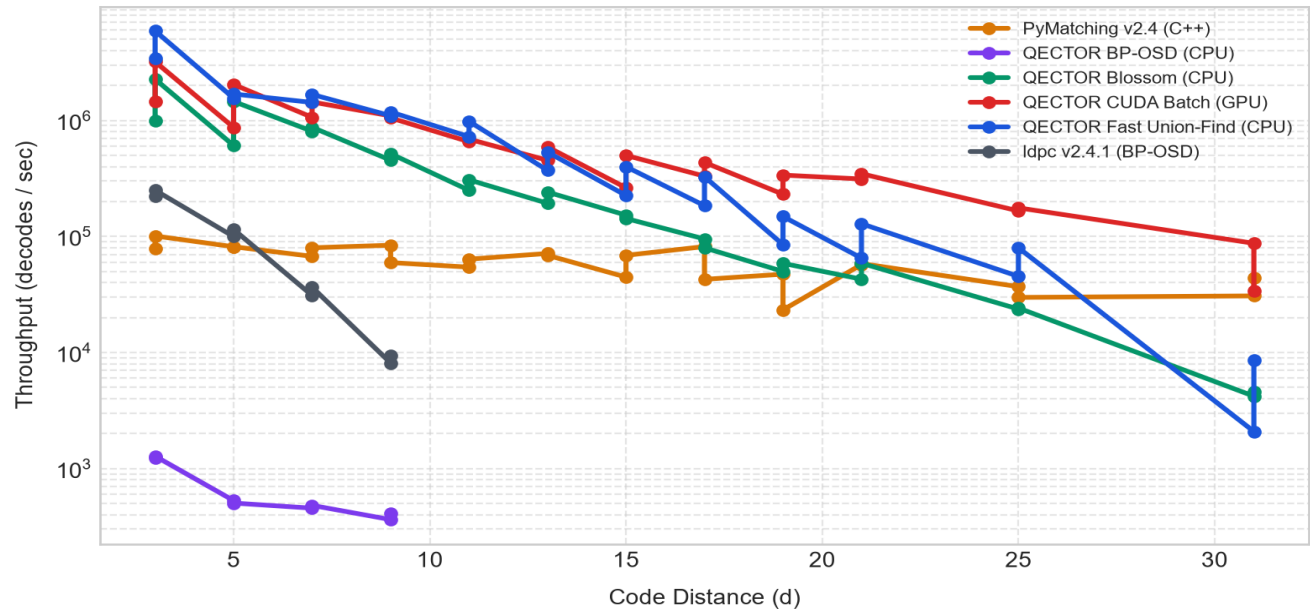
Decoding Throughput vs Code Distance ( d=3..31 )
