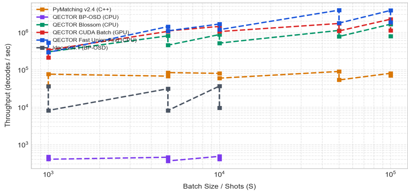
Decoding Throughput vs Batch Size S (1k..100k)
